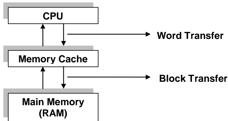
Figure 2.76 “After Cache”
