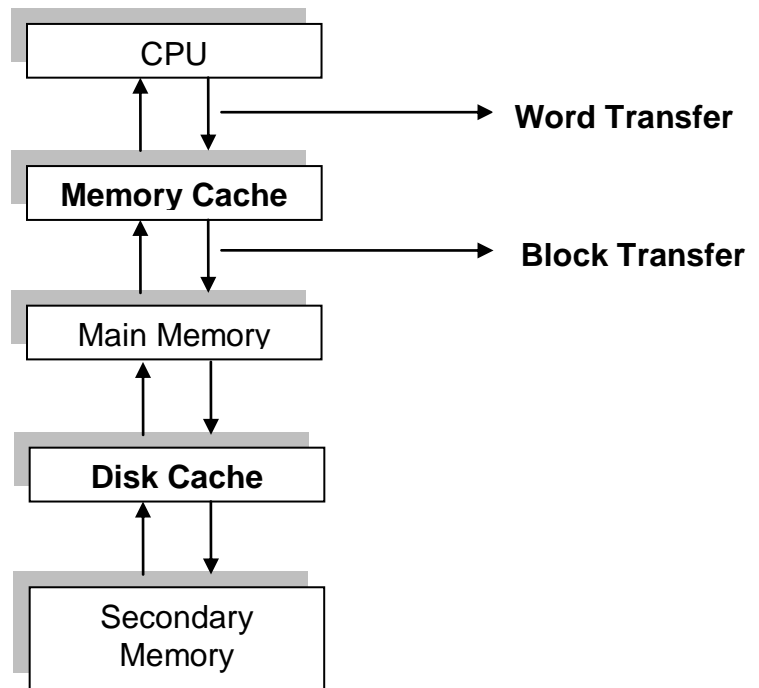
Figure 2.78 "Relationship among CPU, Cache, Main and Secondary Memories"
