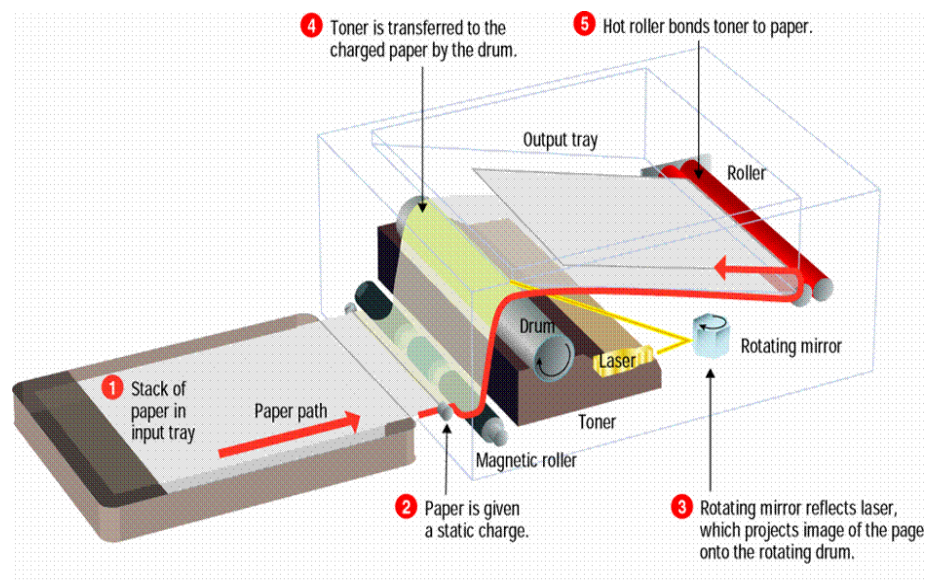
Figure 2.40 "Functionality of LASER Printer"
