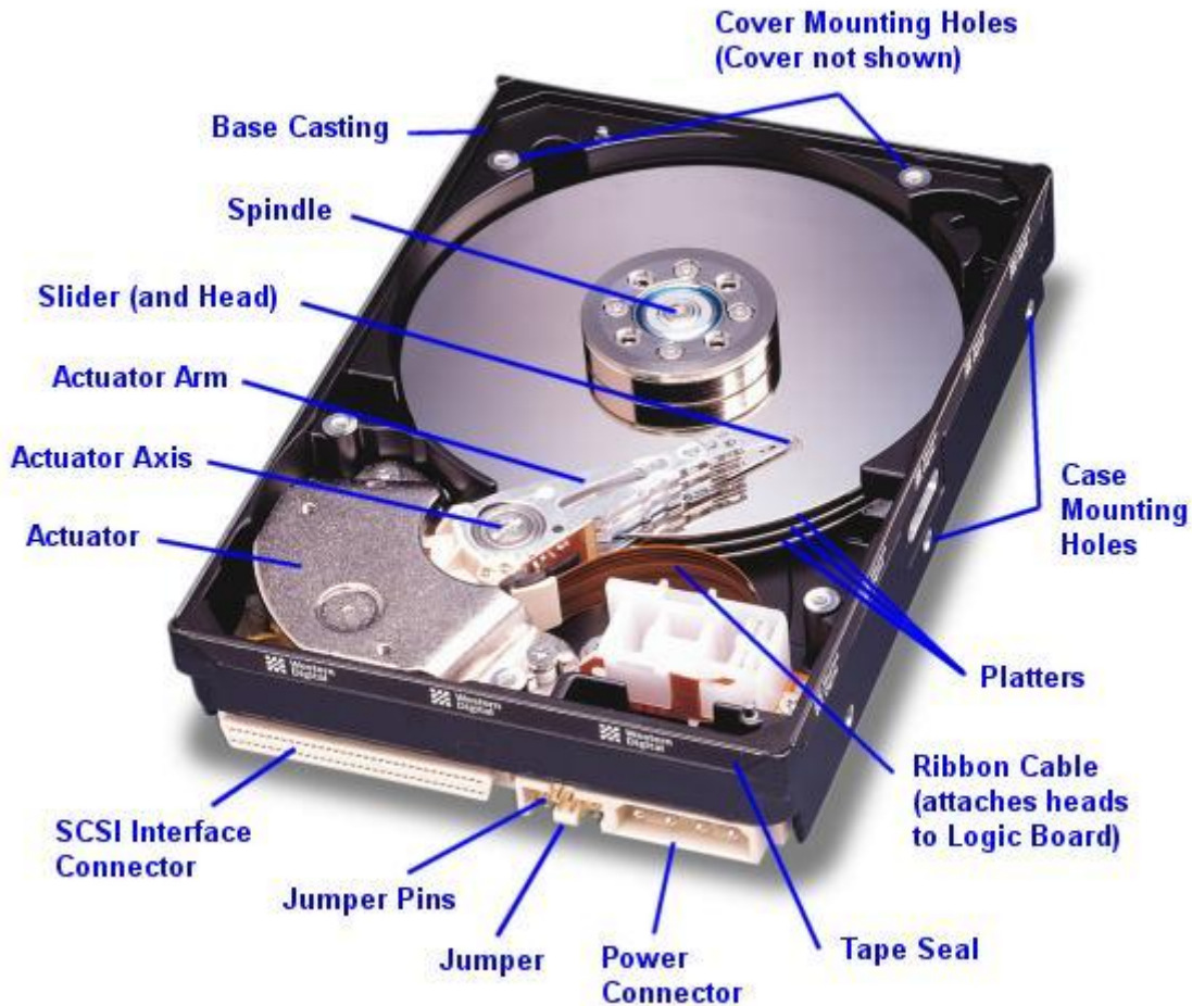
Figure 2.68 "Internal Structure of a Hard Disk"
