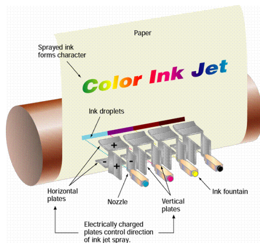
Figure 2.38 "Functionality of Ink-Jet Printer"
