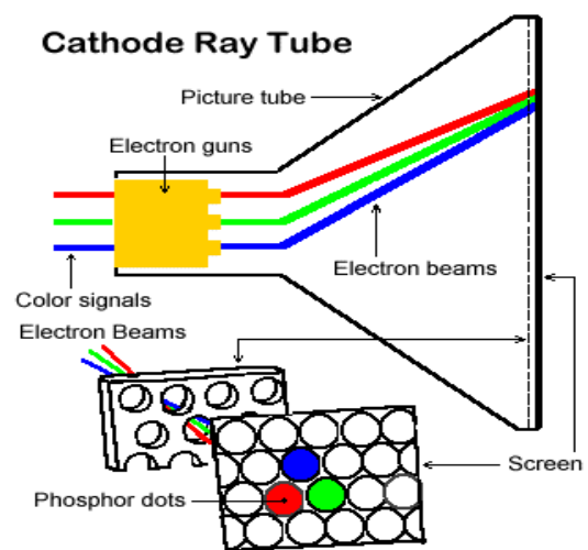
Figure 2.25 “CRT Structure”
