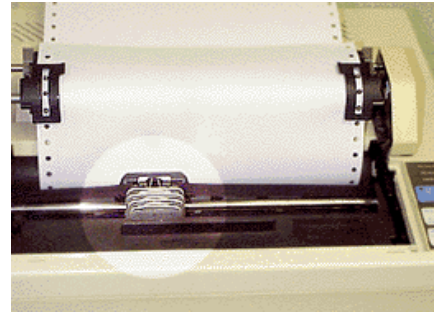
Figure 2.30 "An Impact Printer Showing Detail Of Print Head"
